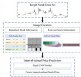
Fig. 3. Dual-CNN 1 based method for interval-valued stock price prediction
