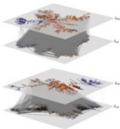
Fig. 1. The multilayer network structure of stock markets in different periods
